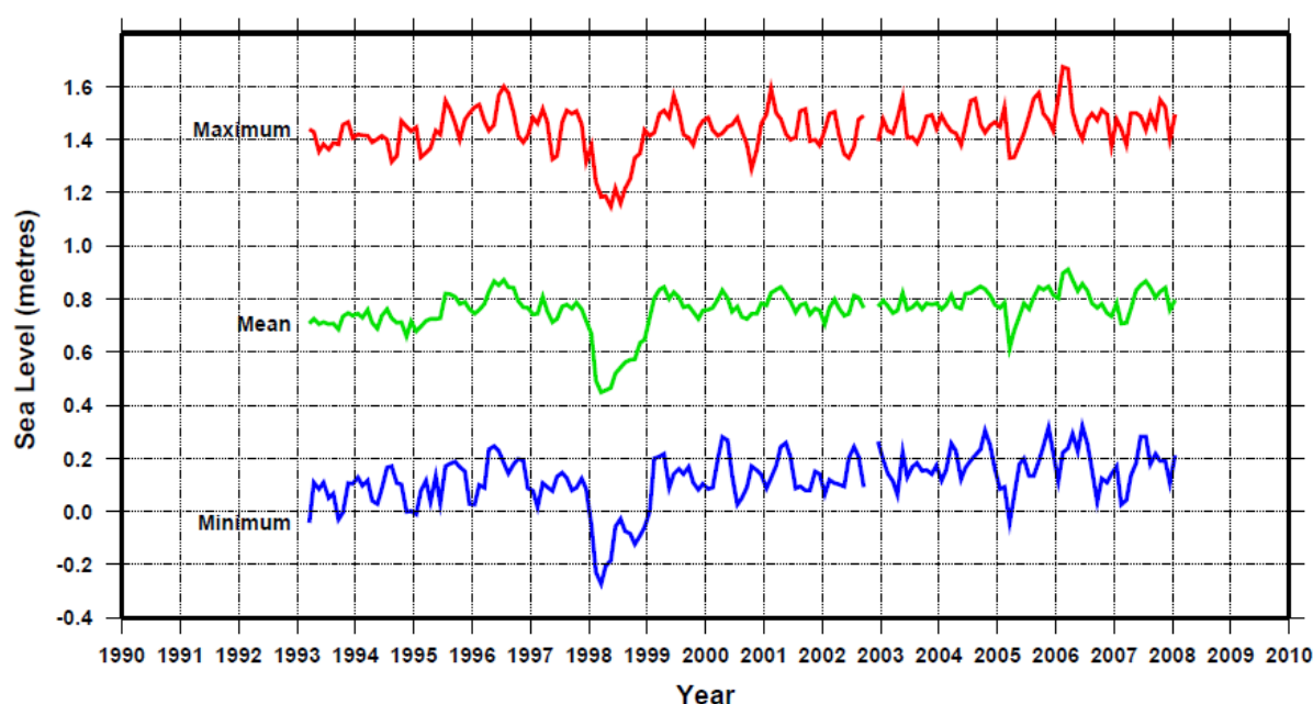
Figure 10. Monthly sea level record from SEAFRAME at Apia, Samoa
