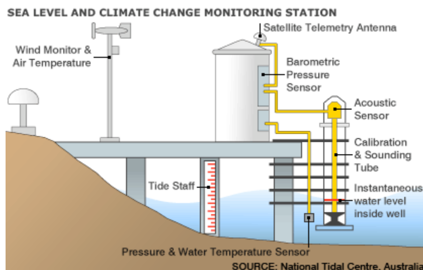
Figure 1. SEAFRAME equipment
