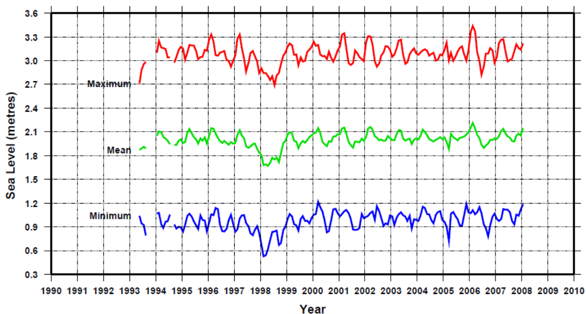
Figure 13 Monthly sea level record from SEAFRAME for Funafuti, Tuvalu
